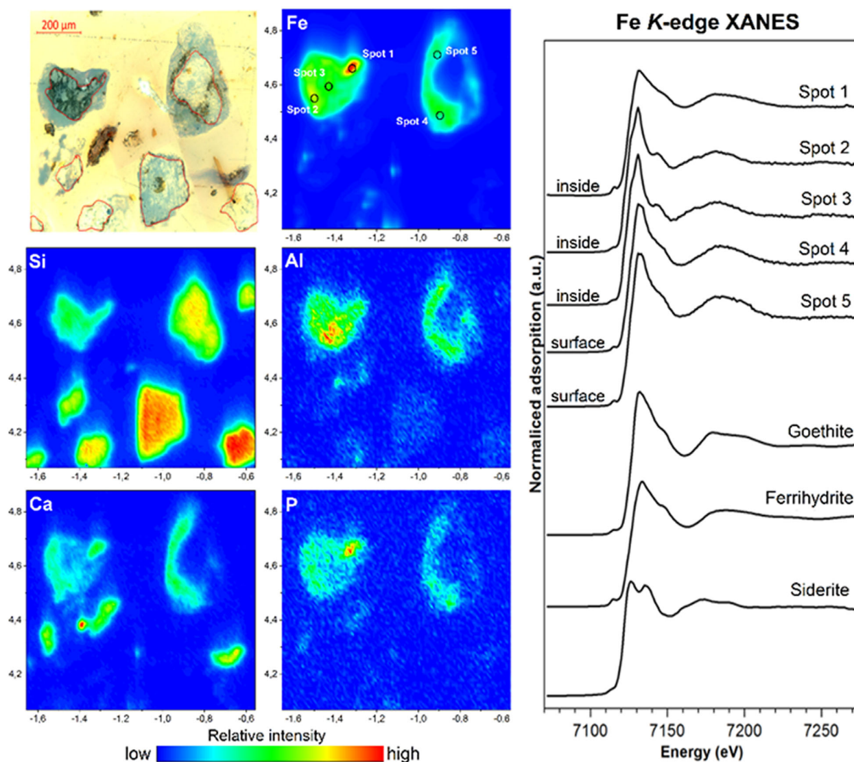
FIGURE 6 Microscopic composite map of large soil microaggregates (53–250 μm) obtained from a Luvisol using reflected and transmitted light microscopic images and respective μ-XRF maps of iron (Fe), silicon (Si), aluminum (Al), calcium (Ca), and phosphorus (P); Fe K-edge μ-XANES spectra of selected spots and exemplary spectra of Fe reference compounds. The μ-XRF maps indicate that the particle in the top left is a composite aggregate, while the rest are primary silicate particles coated with iron and partly phosphorus sorbed to it. Red-bordered parts represent exposed inner parts of aggregates (Kruse et al., unpublished).
